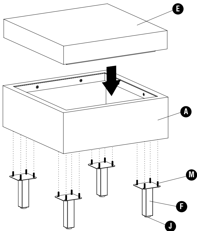
Model MRJLGOU Modèle MRJLGOU Modelo MRJLGOU
