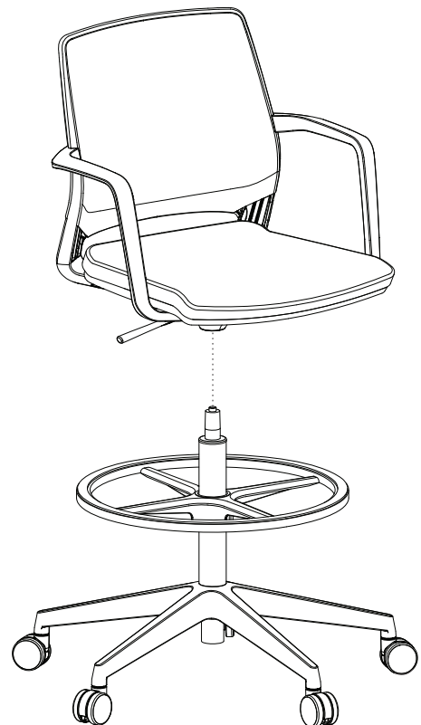
Multi-Purpose Stool shown Tabouret multi-usages illustré Taburete multiusos mostrado
